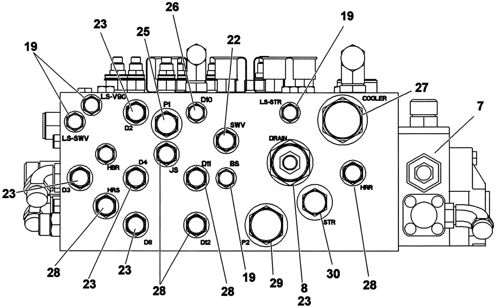
BOTTOM VIEW
